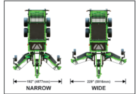
Variable width 192" – 229" (4877- 5816mm) Width adjustment can be done on-the-fly
