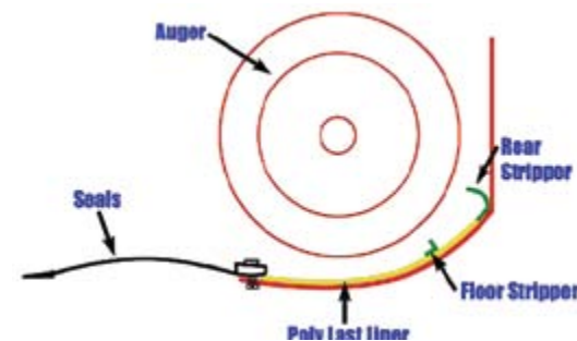
John Deere Liner Detail
