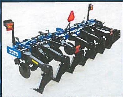
HD Double 7 x 7 Frame with 39" (99 cm) clearance handles high residue and high horsepower of DeepTill
