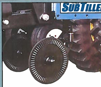
Super 1200 Swivel Coulters and 20" (51 cm) blades slice through heavy BT residue
