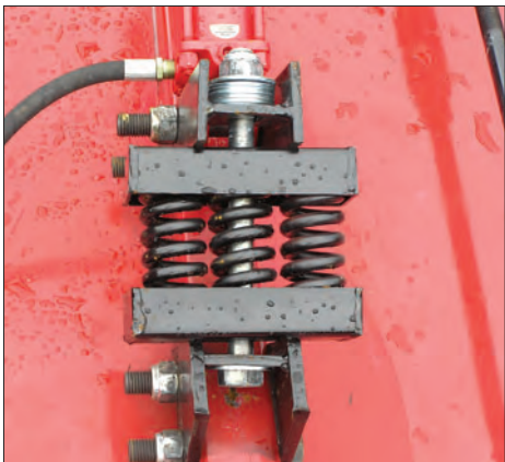
TRIPLE SPRING SHOCK ASSEMBLY (Tailwheel section)
