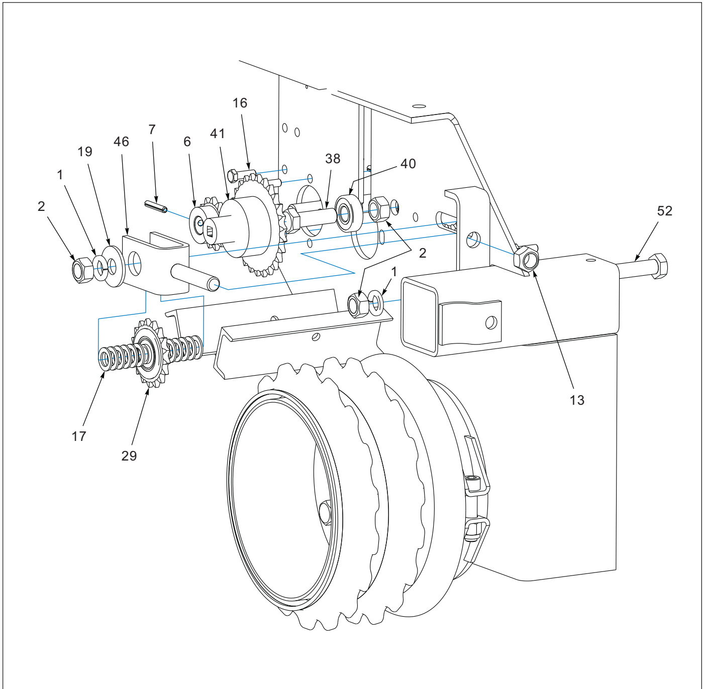
Figure 1-6: Drive Sprockets and Chain Assembly (2 of 2)
