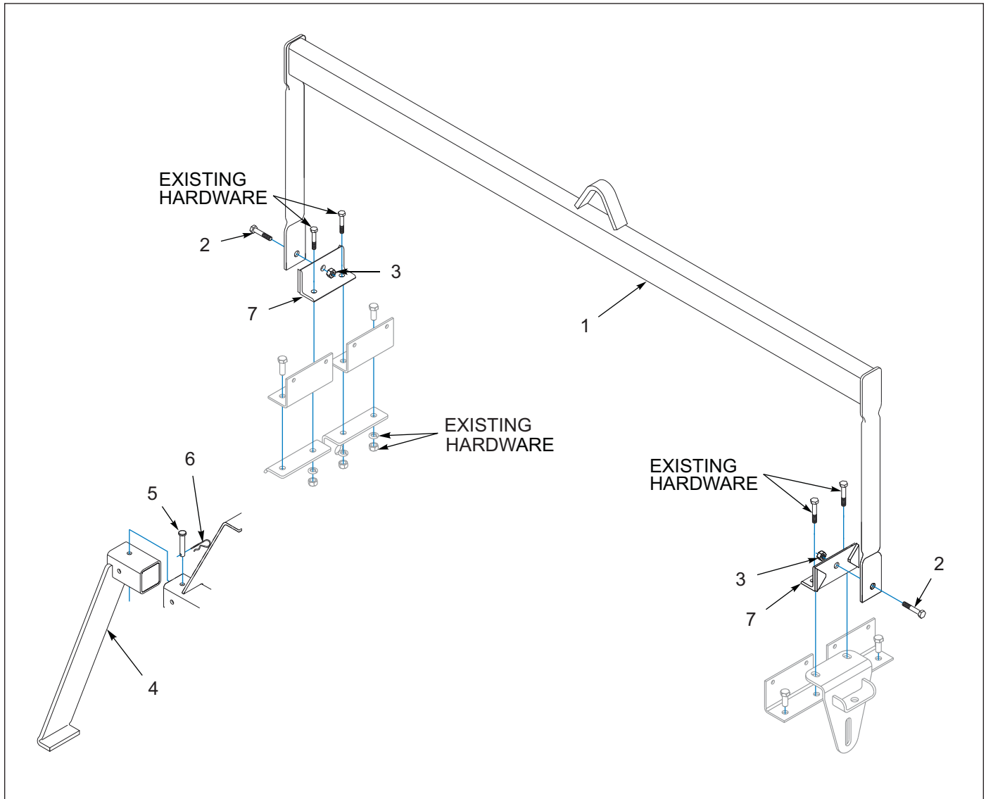
Figure 1-14: Lift Sling Kits
