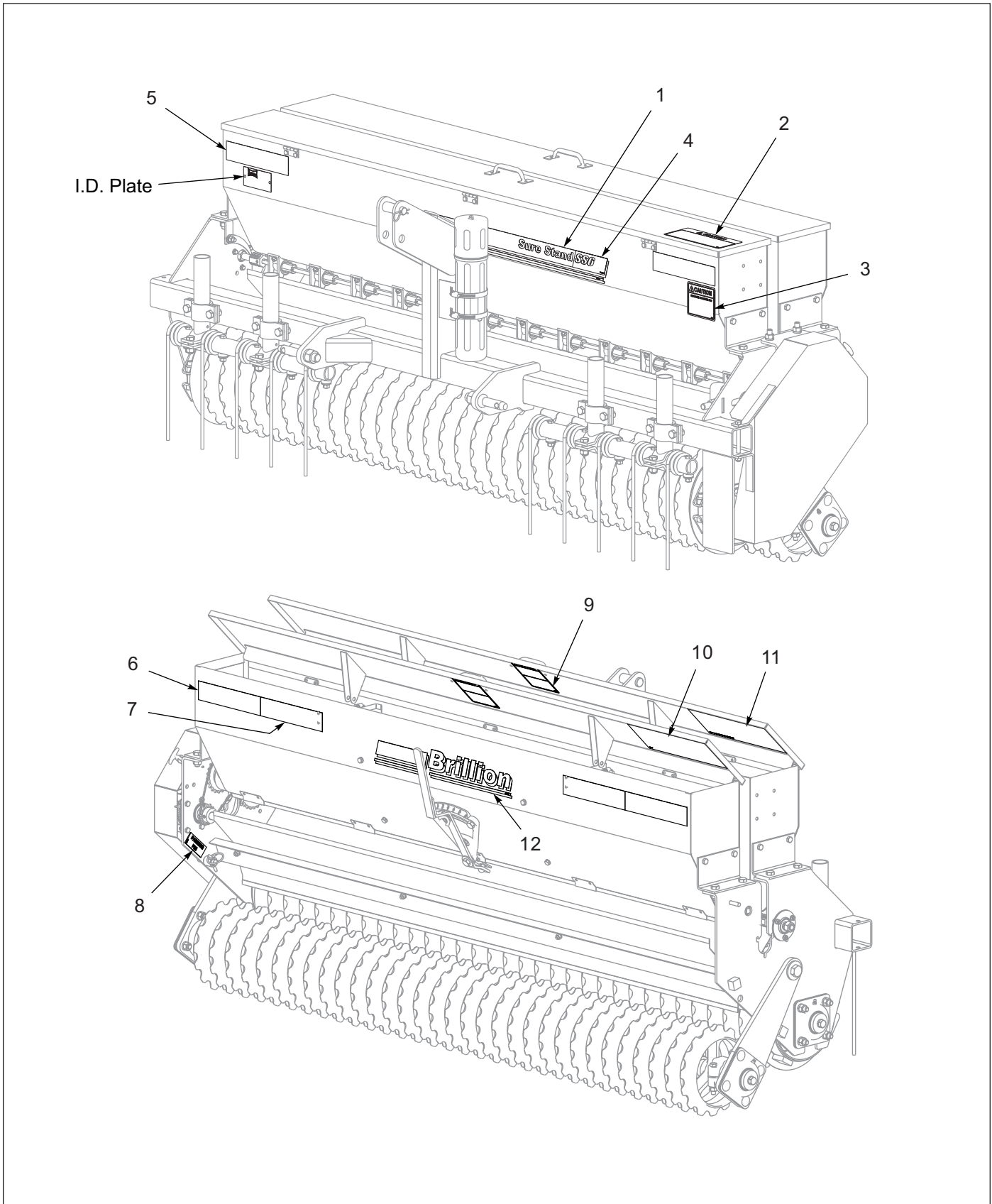
Figure 1-16: Decal Locations
