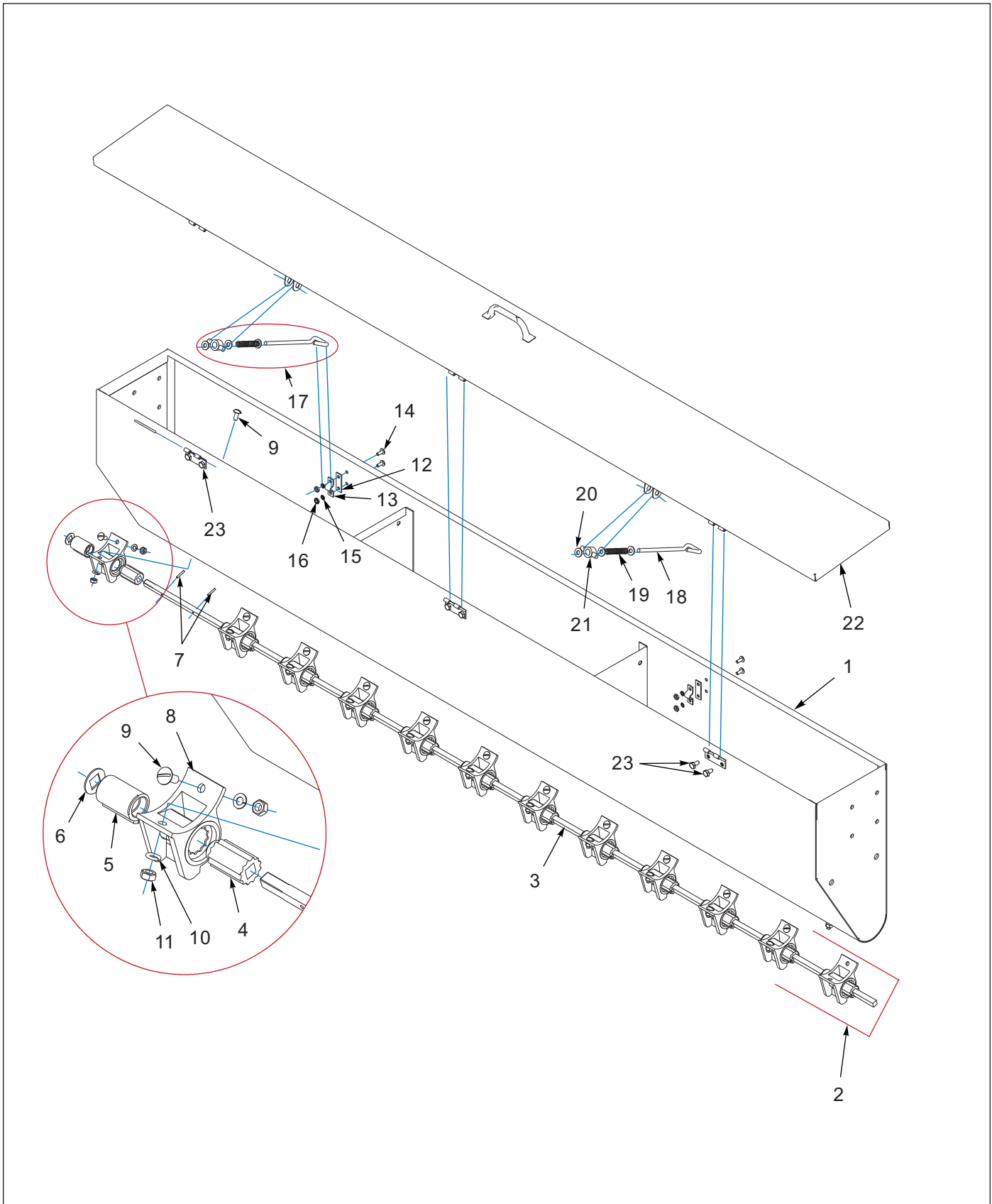
Figure 1-8: Front Seedbox
