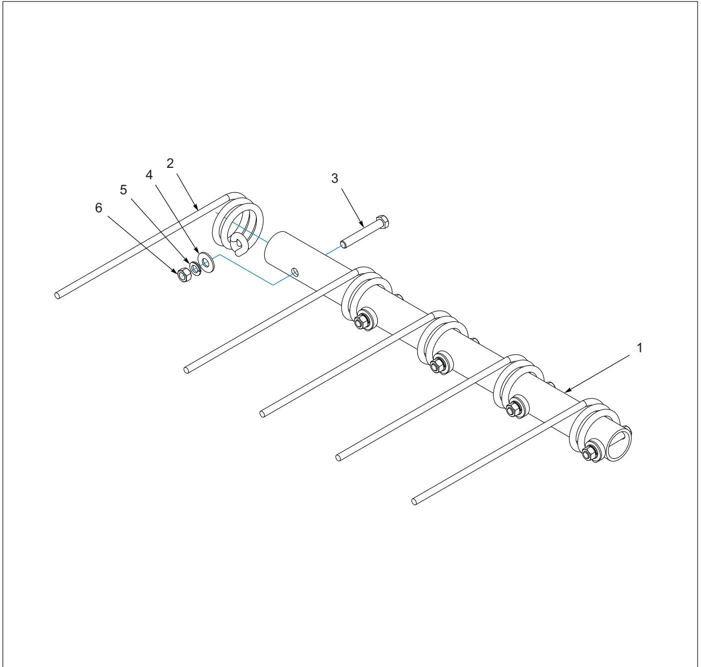
Figure 1-11: Coil Tine Wheel Track Remover 6'
