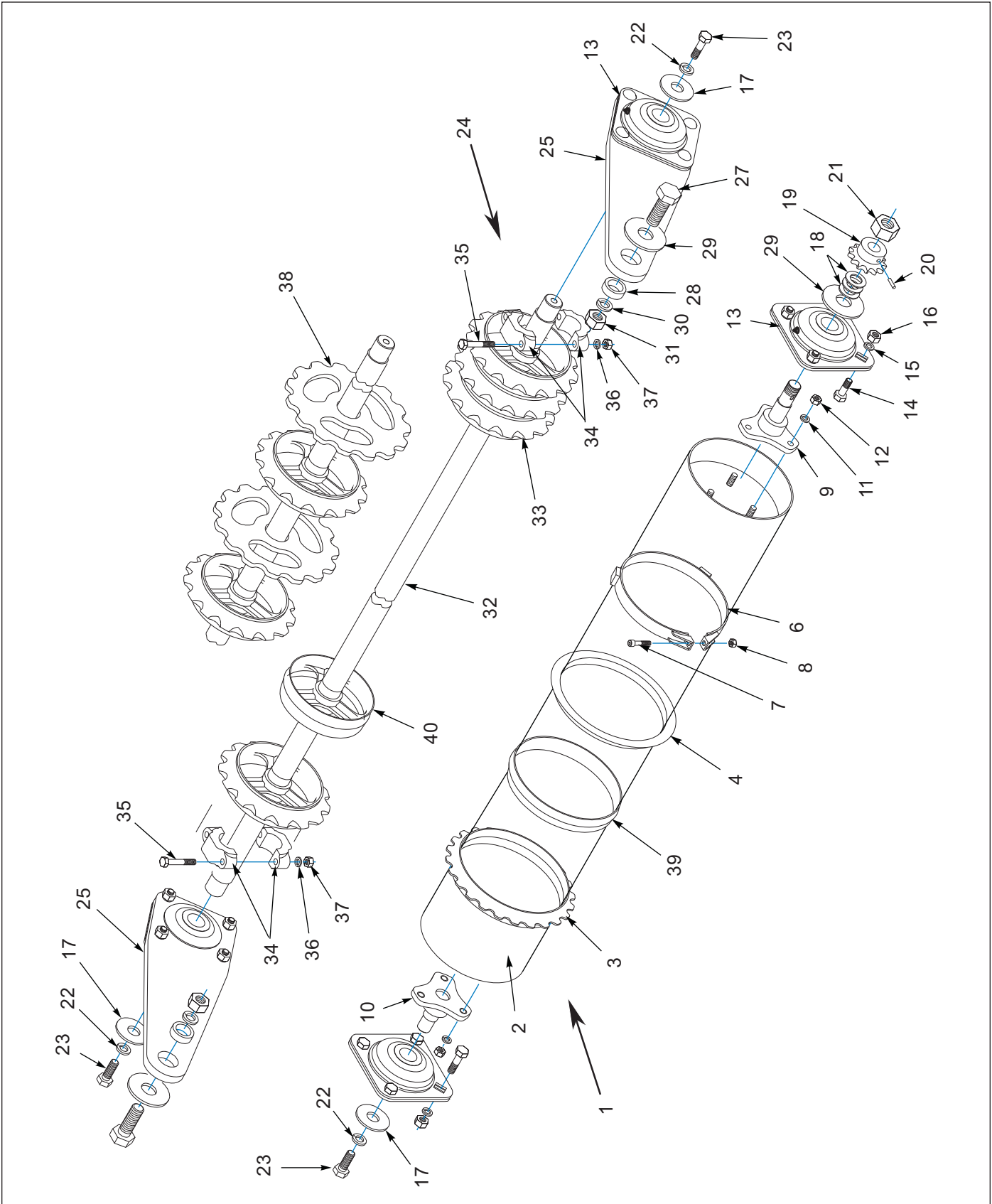
Figure 1-4: Wheel and Axle Assemblies
