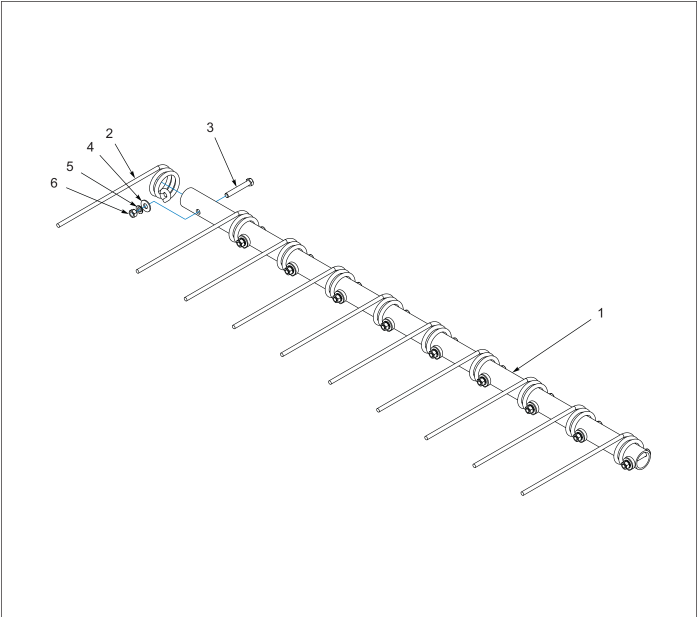
Figure 1-10: Coil Tine Wheel Track Remover 4' and 5'
