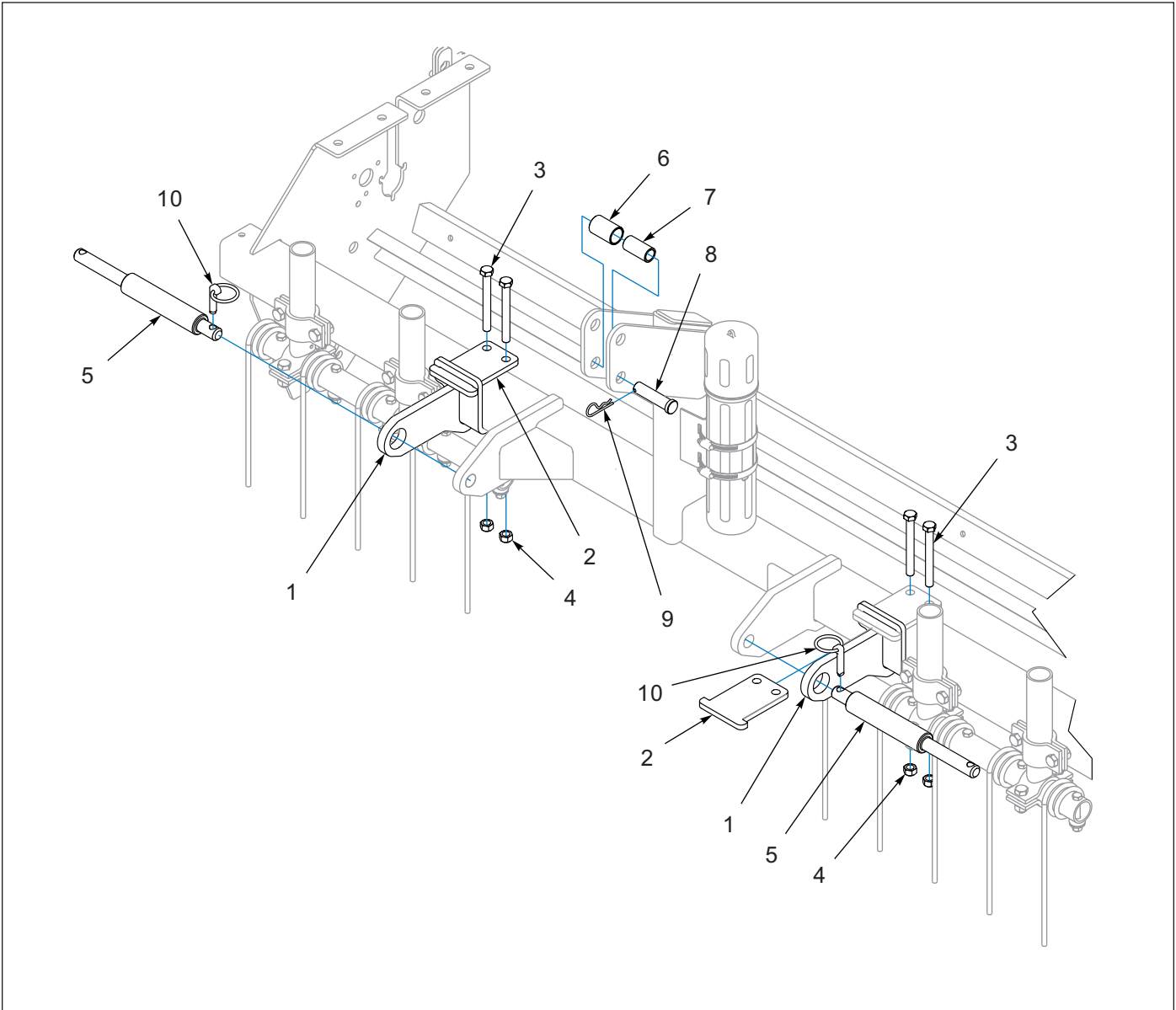
Figure 1-13: CAT2 Quick Coupler Hitch Adaptor Kit - Optional
