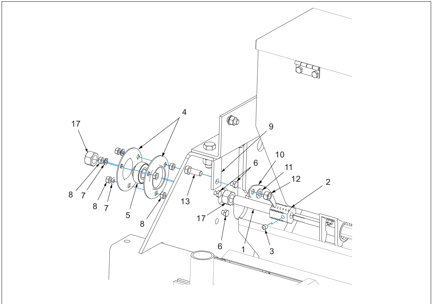
Figure 1-7: Right End Components
