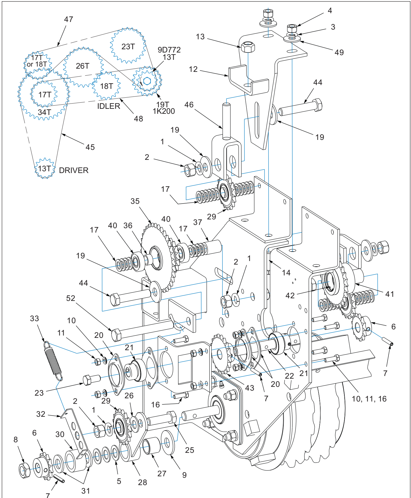
Figure 1-5: Drive Sprockets and Chain Assembly (1 of 2)
