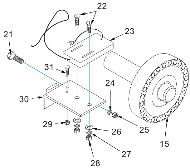
Figure 1-12: Electric Acre Meter Assembly
