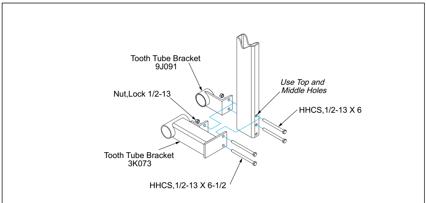
Figure 2-12: S - Tine Bracket Assembly
