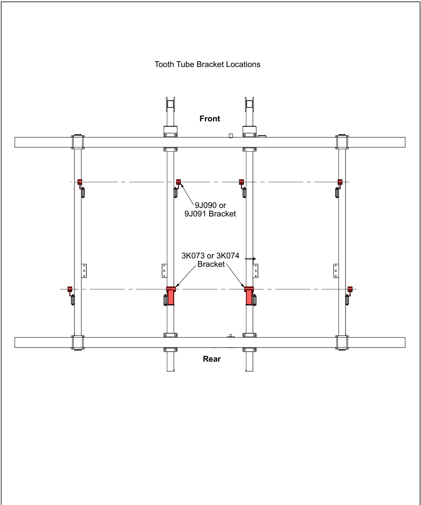
Figure 2-13: Tooth Tube Bracket Locations
