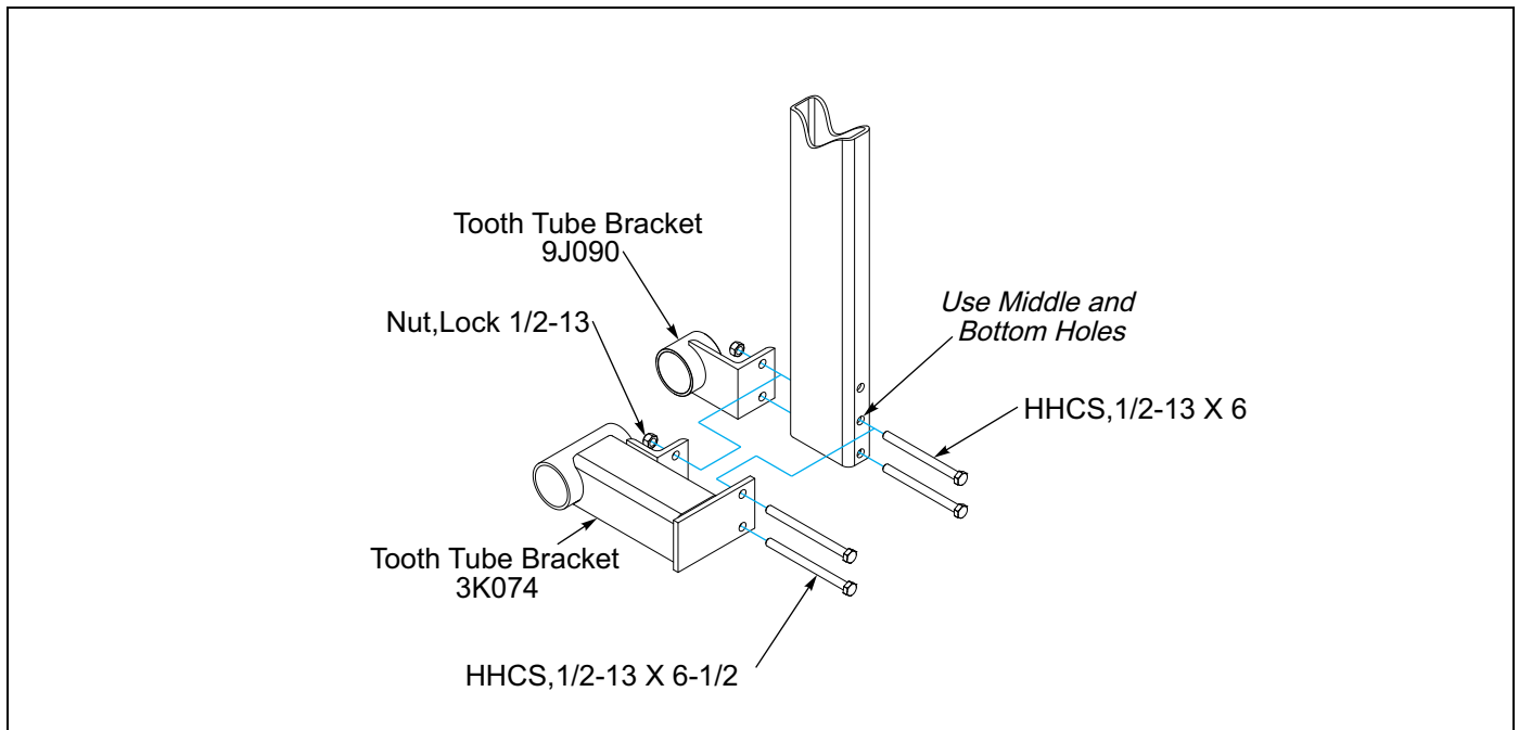
Figure 2-11: C - Tooth Bracket Assembly
