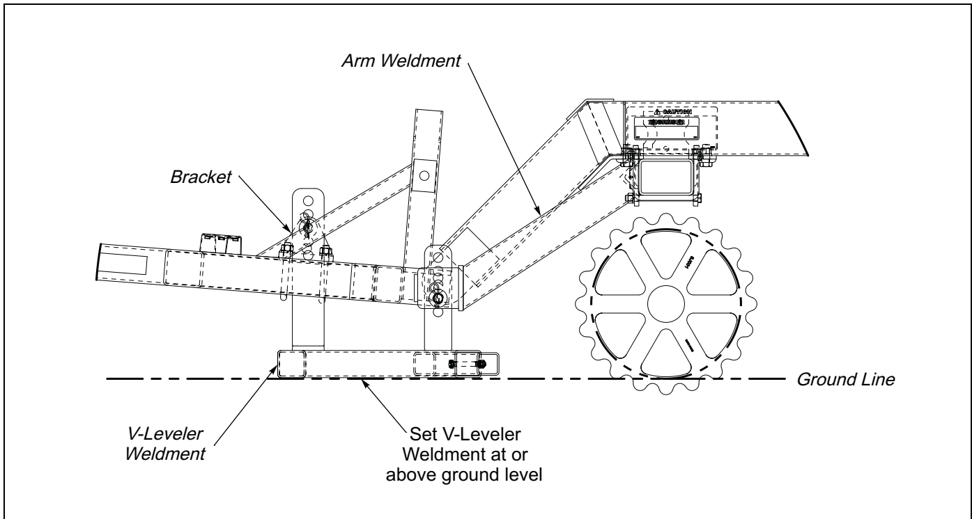
Figure 3-7: V-Leveler Side View
