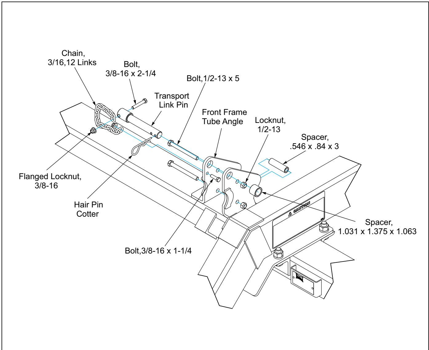
Figure 2-4: Transport Link Pin Installation
