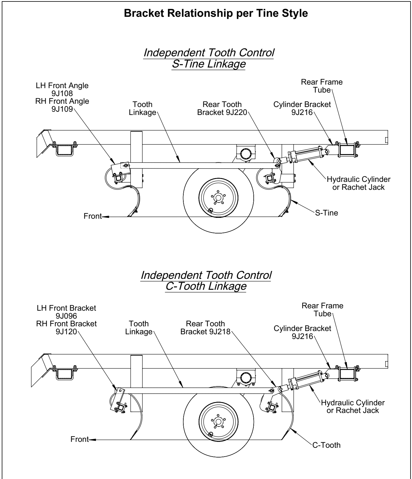
Figure 2-21: Bracket Relationship per Tine Style - Independent
