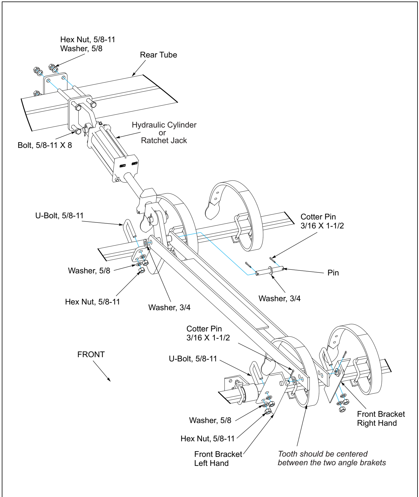
Figure 2-19: Independent Tooth Control C-Tooth Installation
