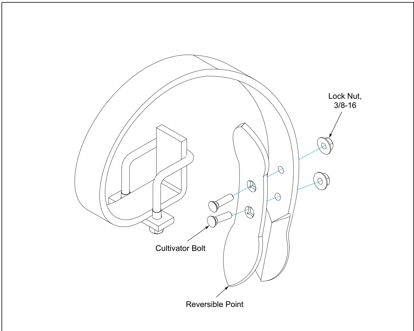
Figure 4-4: C-Tooth Point Replacement
